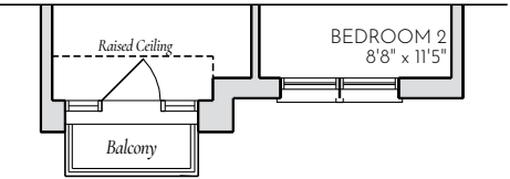
PART. UPPER FLOOR ELEV. 'A2'
