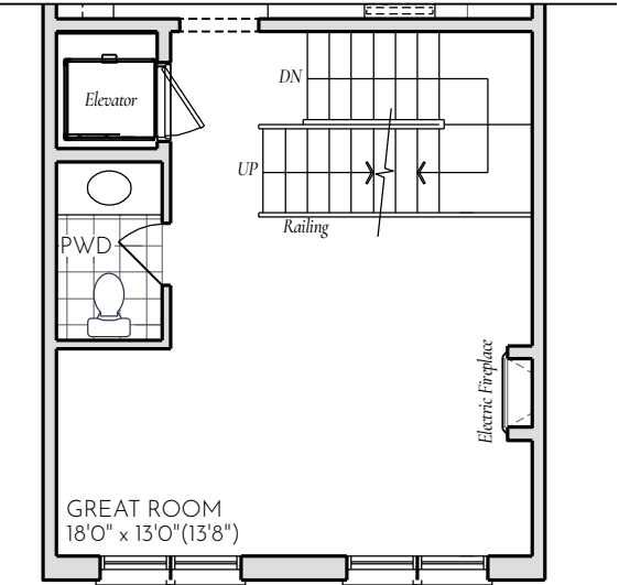
PART. MAIN FLOOR OPT. ELEVATOR ELEV. 'A1' (OTHER ELEV. SIMILAR)
