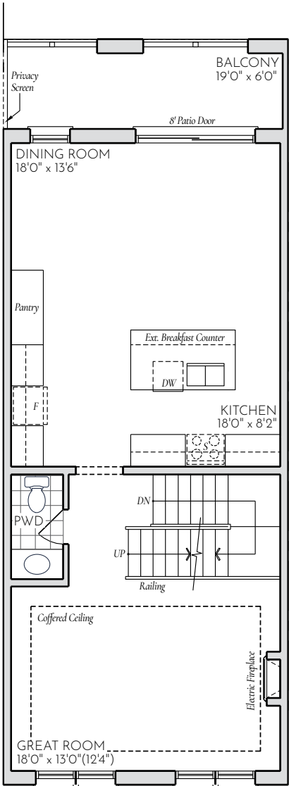
MAIN FLOOR ELEV. 'A1'
