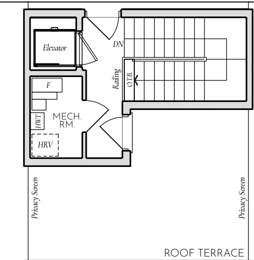
ROOF TERRACE OPT. ELEVATOR ELEV. 'A1' (OTHER ELEV. SIMILAR)
