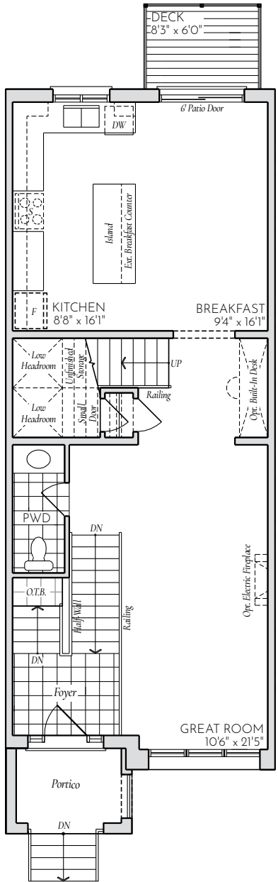
MAIN FLOOR ELEV. 'A1'
