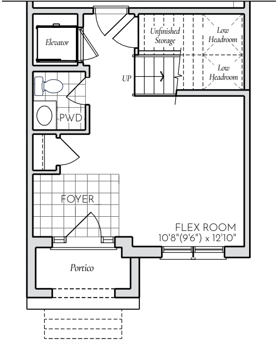
PART. LOWER FLOOR OPT. ELEVATOR ELEV. 'A1' (OTHER ELEV. SIMILAR)
