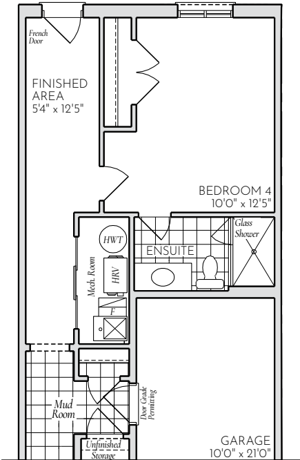
PART. OPT. LOWER FLOOR ELEV. 'A1' W/ BEDROOM (A2' SIMILAR)
