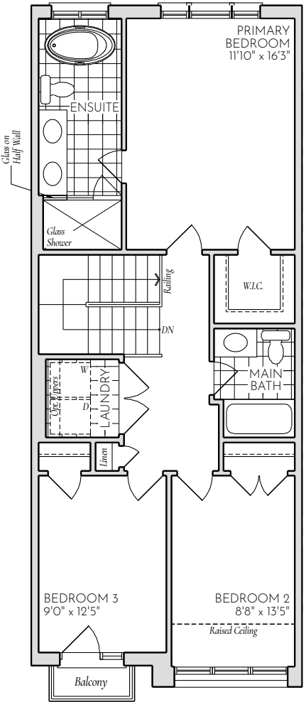
UPPER FLOOR ELEV. 'A1'
