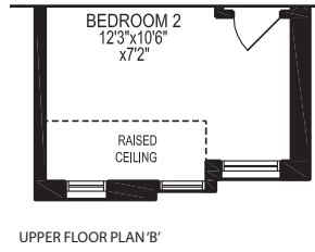
UPPER FLOOR PLAN 'B'
